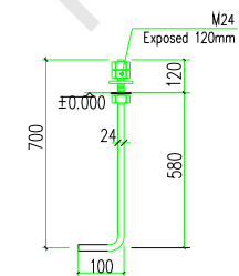
The Anchor Bolt Plan
